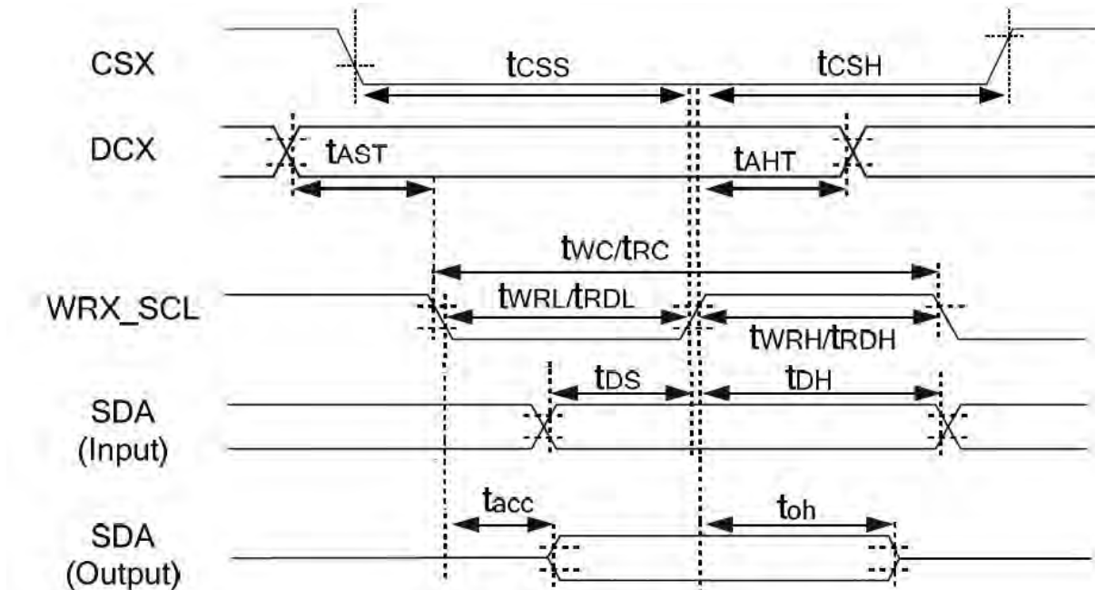
Figure 8.2: SPI interface characteristics
