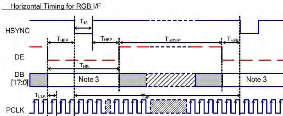
Figure 8.4: General timings for RGB I/F-2
