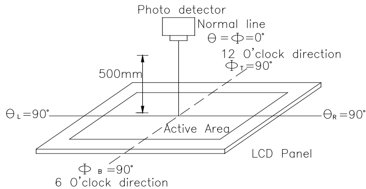
Fig. 9.2. Optical measurement system setup
