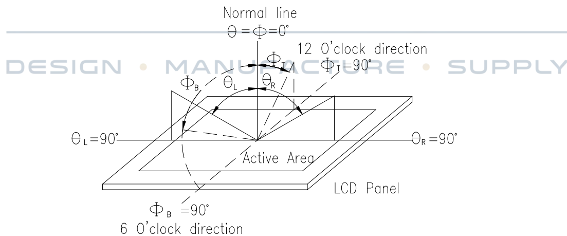
Fig. 9.1. Definition of viewing angle
