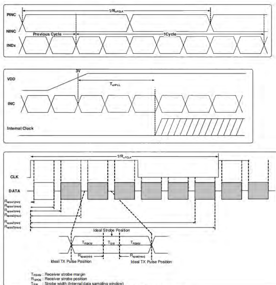
Figure 13.3: LVDS figure
