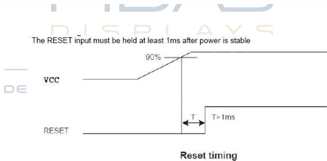
Figure 3. 2 Vertical input timing diagram.
