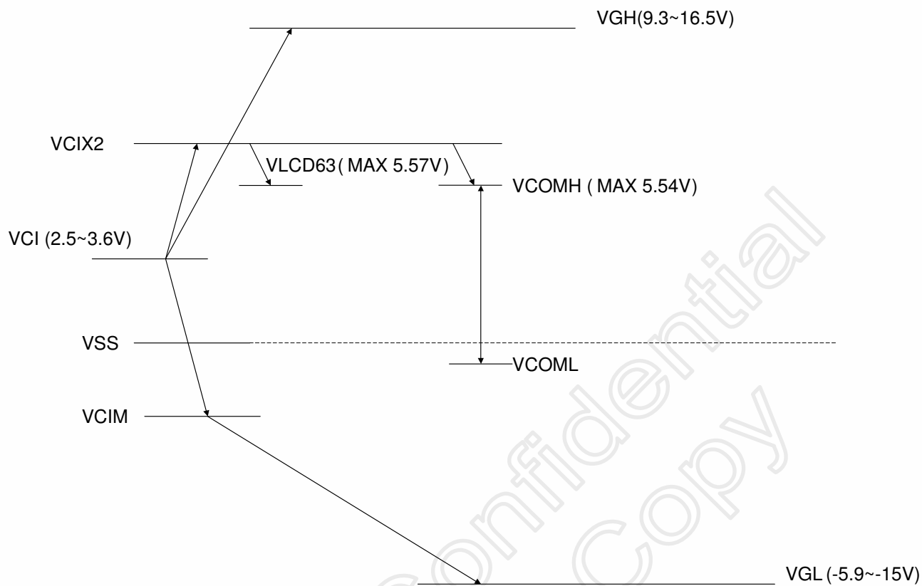
Figure 15. 1 LCD driving voltage relationship
