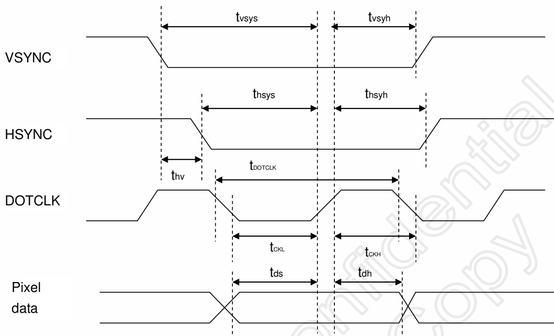
Figure 14. 1 Pixel timing
