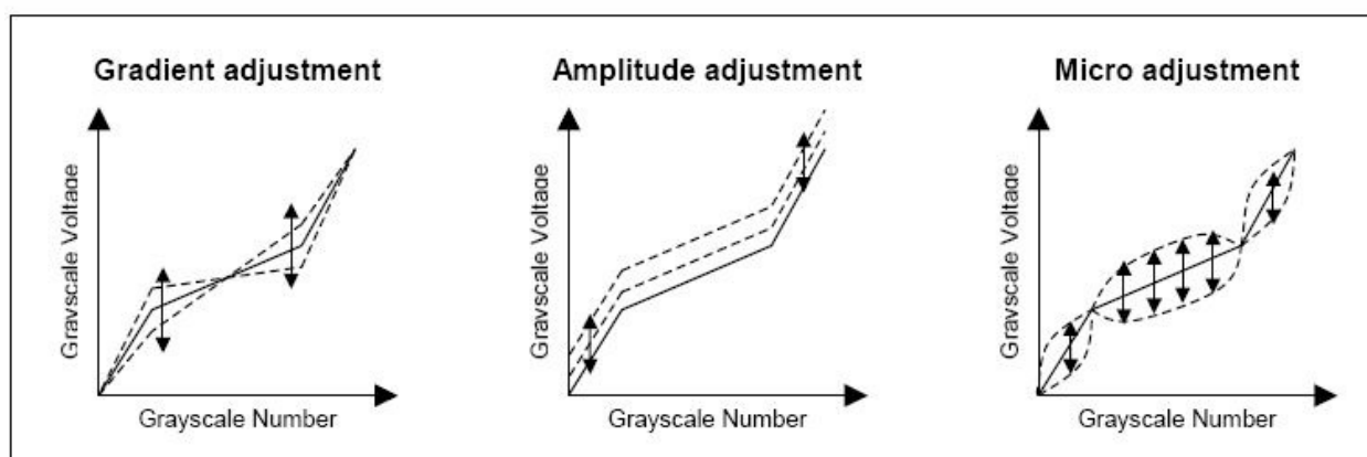
Figure 11. 4 Gamma adjustment function
