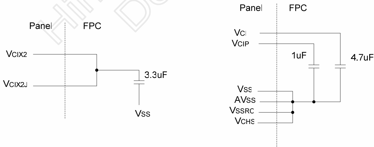
Figure 16.4 Panel and FPC connection
