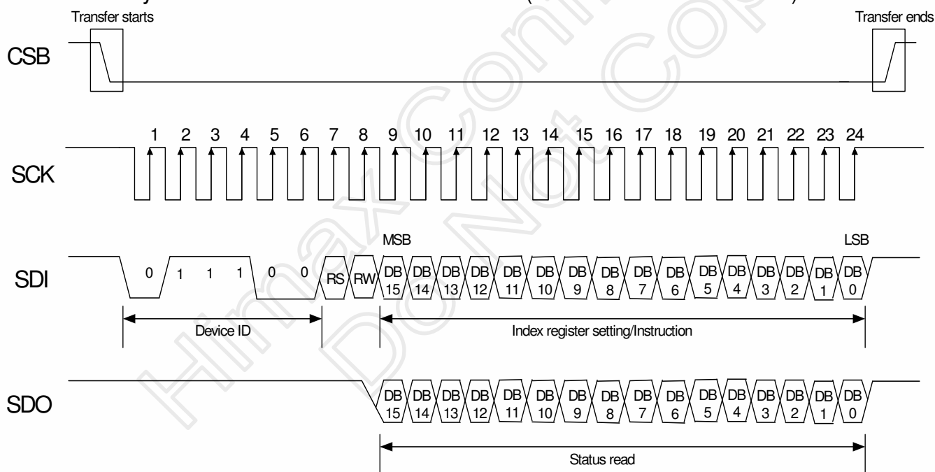
Figure 7.1 SPI Timing
