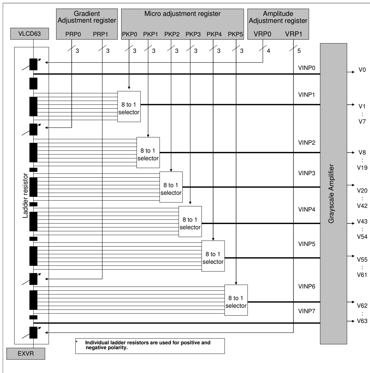
Figure 11. 2 Grayscale amplifier
