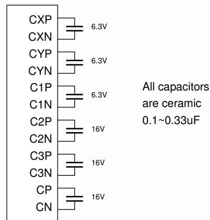
Figure 16.1 Booster capacitors
