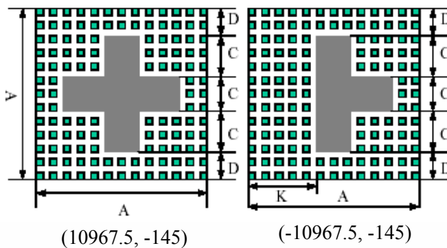
Figure 4. 1 HX8238-A die floor plan (bump face up)
