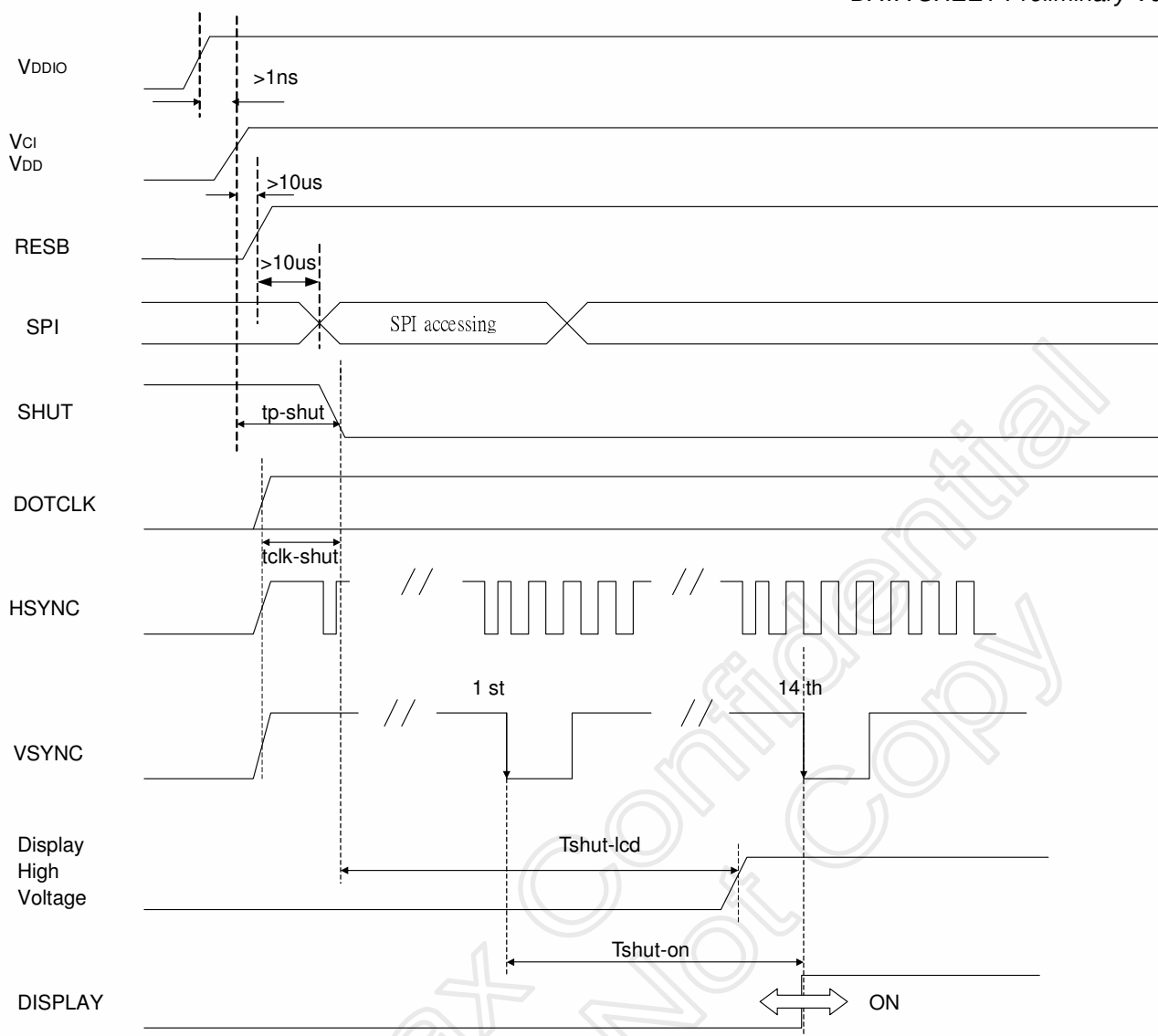
Figure 14. 10 Power up sequence
